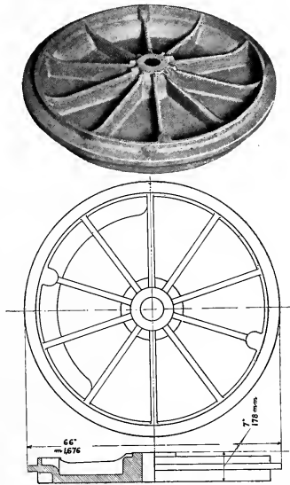
Fig. 15. Marine Engine Cylinder Head—Weight 2400 pounds.
